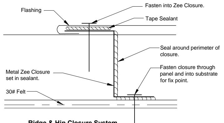
Ridge & Hip Closure System 10' metal Zee closure.
